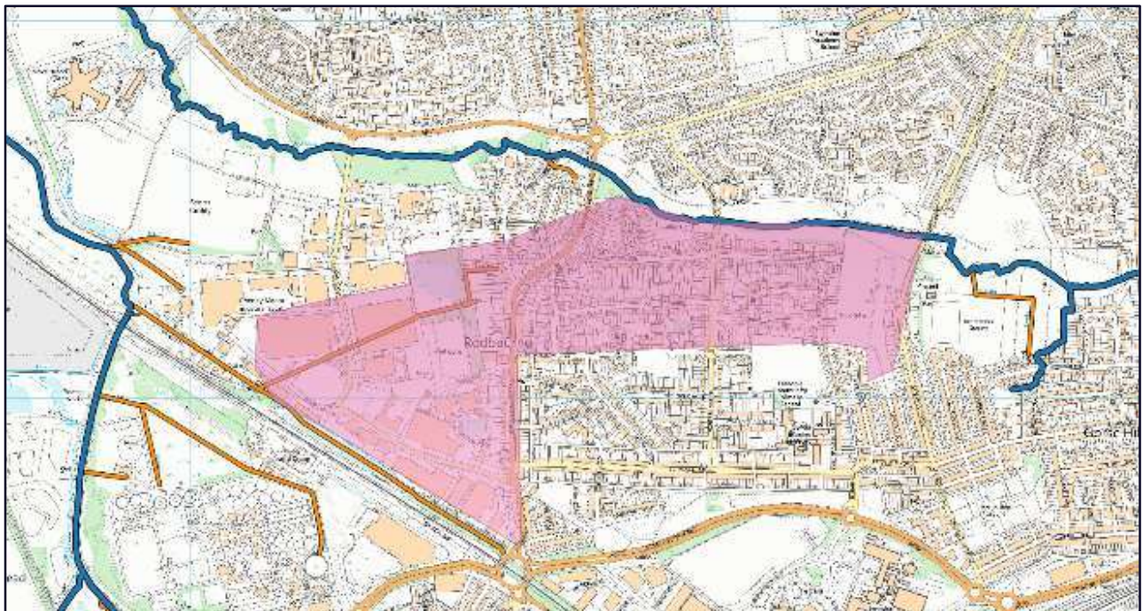
Figure 25 Rodbourne Cheney High Priority Area (Pink) Main River (Blue) and Ordinary Watercourses (Orange)
