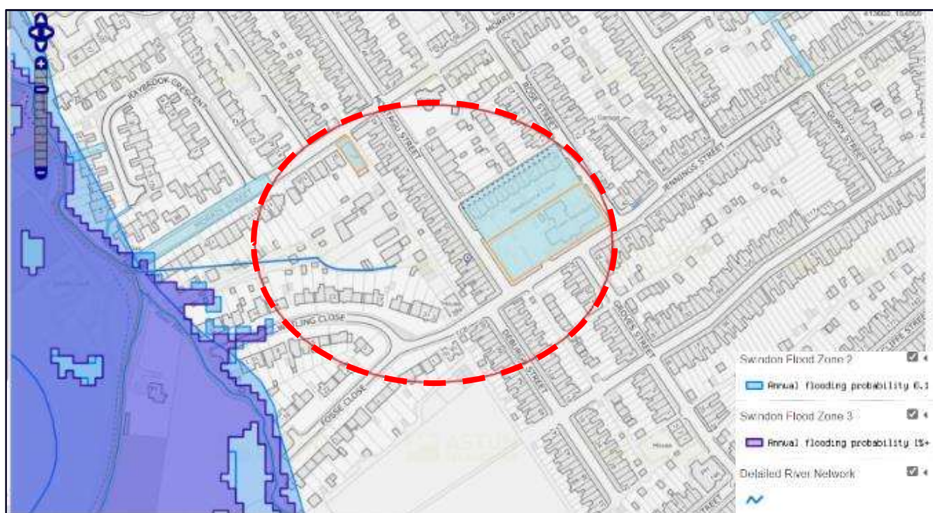
Figure 19 Fluvial Flood Risk Map (showing section of ordinary watercourse to the rear of Montagu Street properties (enclosed in red circle)
